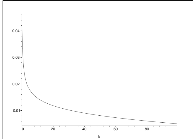
Figure 3: Plot of \mathcal{B}(p_t)/|t| as a function of k ( N = 100 ).
