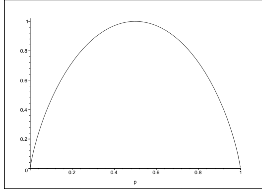
Figure 1: Binary entropy function \mathcal{B}(p) in [0, 1]
