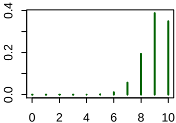
p = 0.9, n = 10
