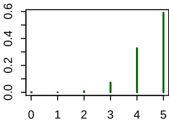
p = 0.9, n = 5
