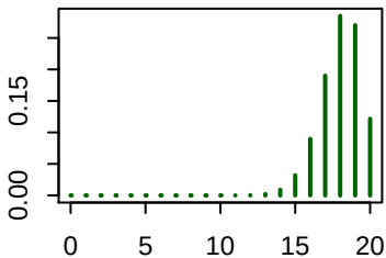
p = 0.9, n = 20
