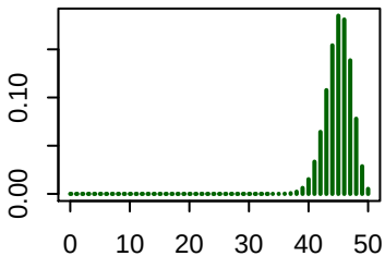
p = 0.9, n = 50
