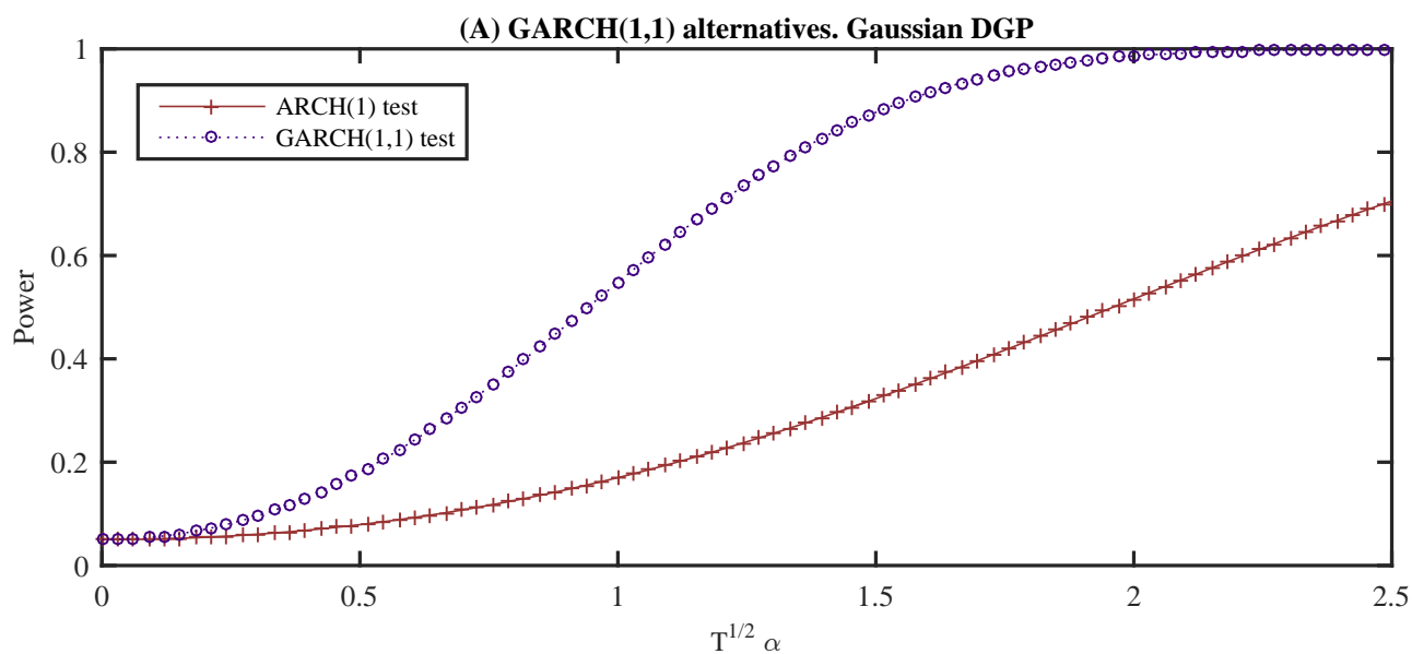
FIGURE 6: Local power of unpredictability in variance tests at 5% level
